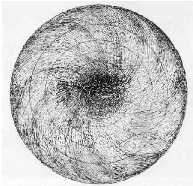
Plate 23. EARTH. Black center, and her atmosphere.
