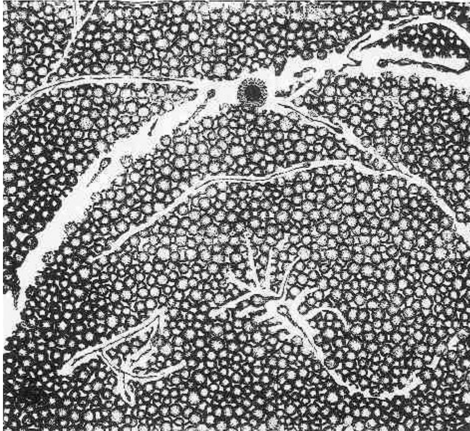
Plate 21. THE EARTH IN THE ARC OF BON.
