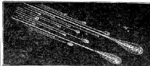
FIRE-BALL (as observed in a Telescope).
