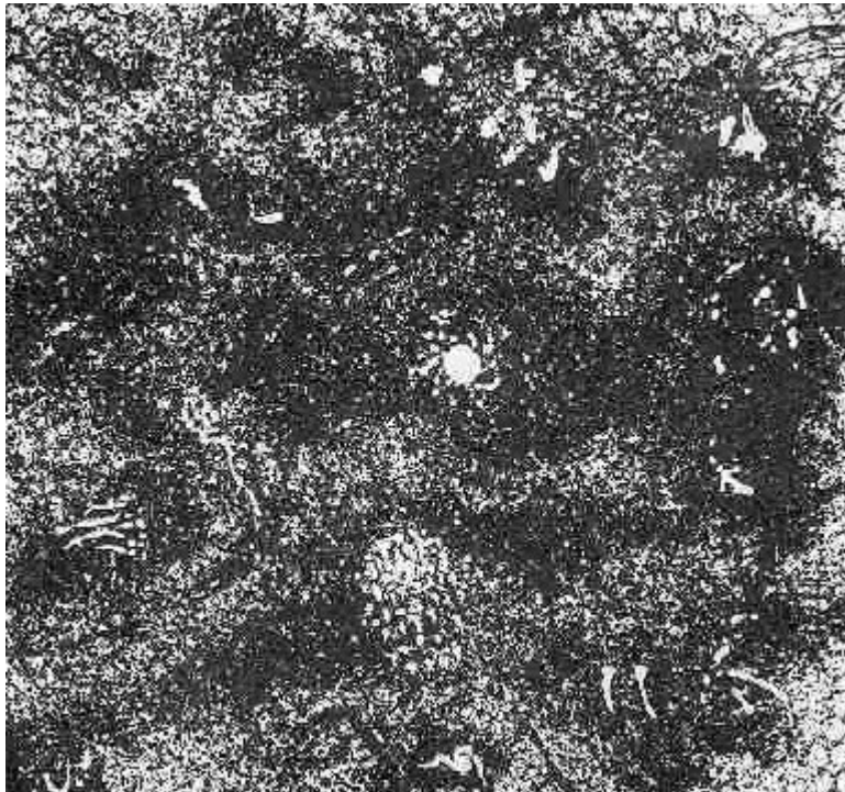
Plate 32. THE EARTH IN A'JI.
