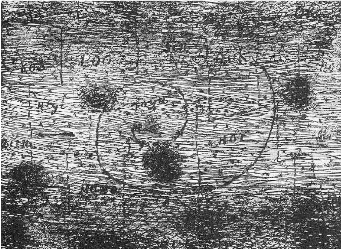
Plate 39. THE EARTH IN SE'MU.
