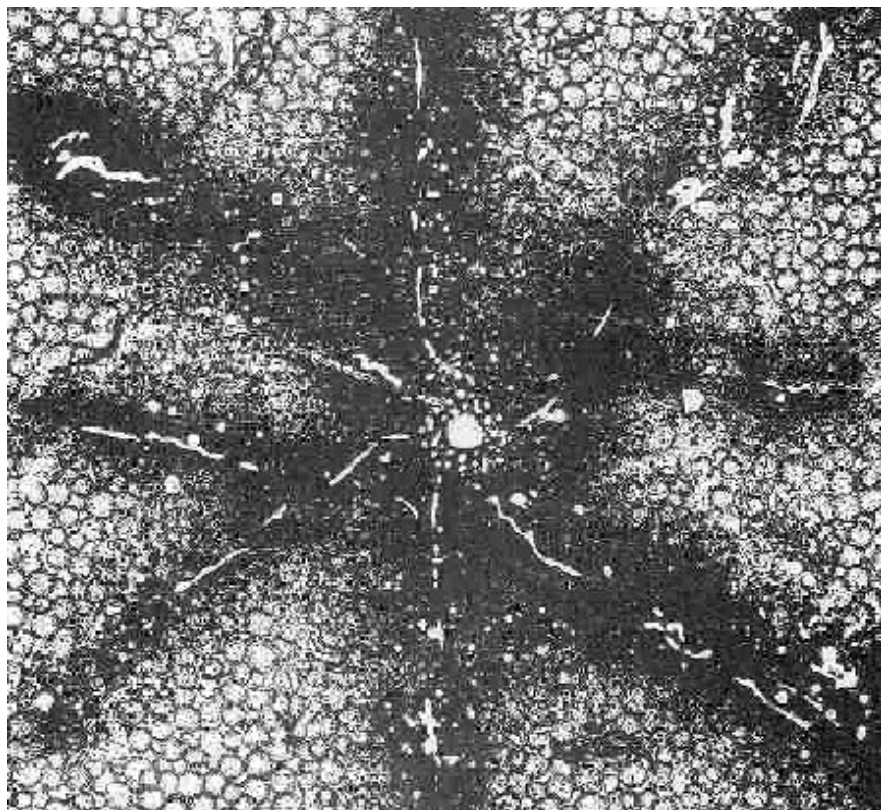
PLATE 30. JI'AY. The earth (white spot) in Ji'ay.
