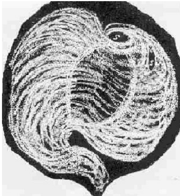
Plate 28. FOURTH AGE OF VORTEX. Now called Inqua, a ball within a ball, or womb of vapor. ( S, S, satellites ).
