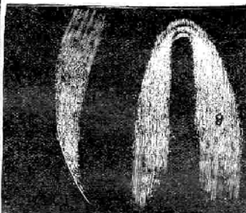
DONATI'S COMET. (General view.) DONATI'S COMET. (Showing the head and envelope.)
