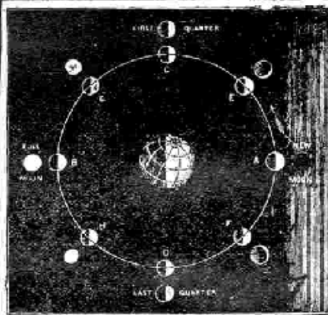
THE PHASES OF THE MOON.
