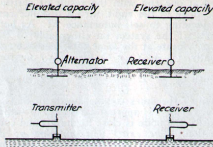
Transmission of Electrical Energy Thru the Earth as Illustrated in Tesla's Lectures Before the Franklin Institute and Electric Light Association in February and March, 1893, and Mechanical Analog of the Same. Fig. 7.
