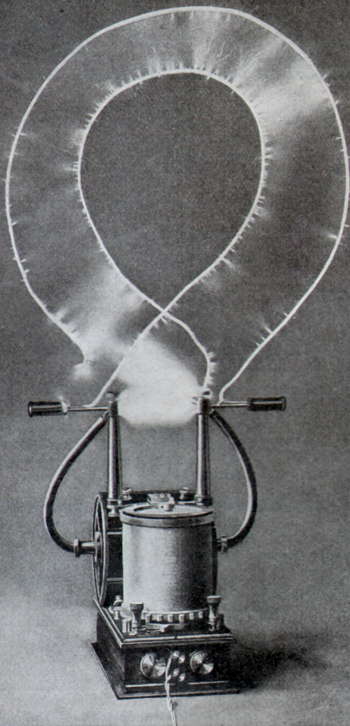
Fig. 1—Tesla Oscillation Transformer (Tesla Coil) Presented by Lord Kelvin Before the British Association in August, 1897. This Small and Compact Instrument, Only 8 Inches High, Developed Two Square Feet of Streamers With Twenty-Five Watts From the 110 Volt D. C. Supply Circuit. The Instrument Contains a Tesla Primary and Secondary, Condenser, and a Circuit Controller.
